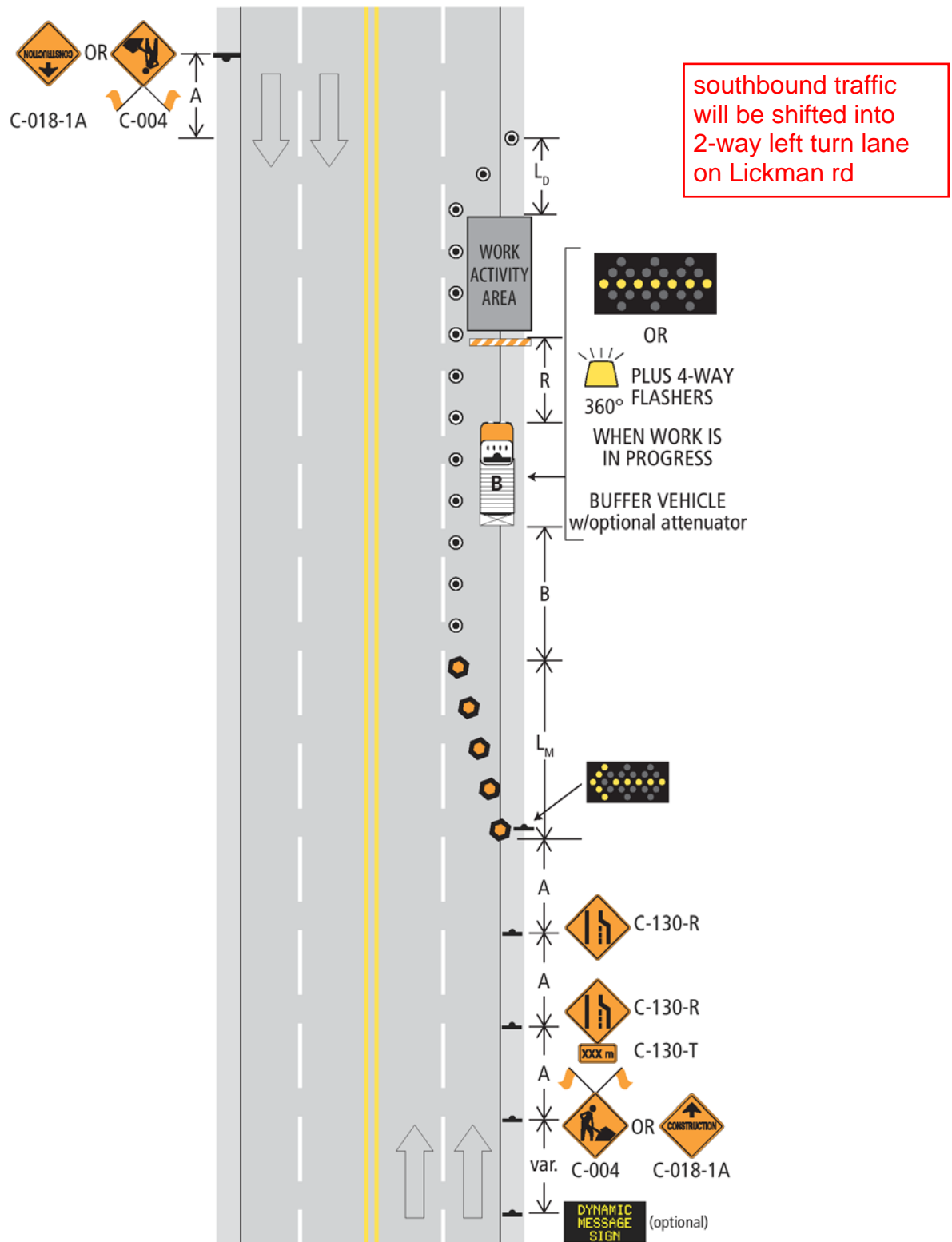
Figure 8.6: Right Lane Closed – Short and Long Duration
